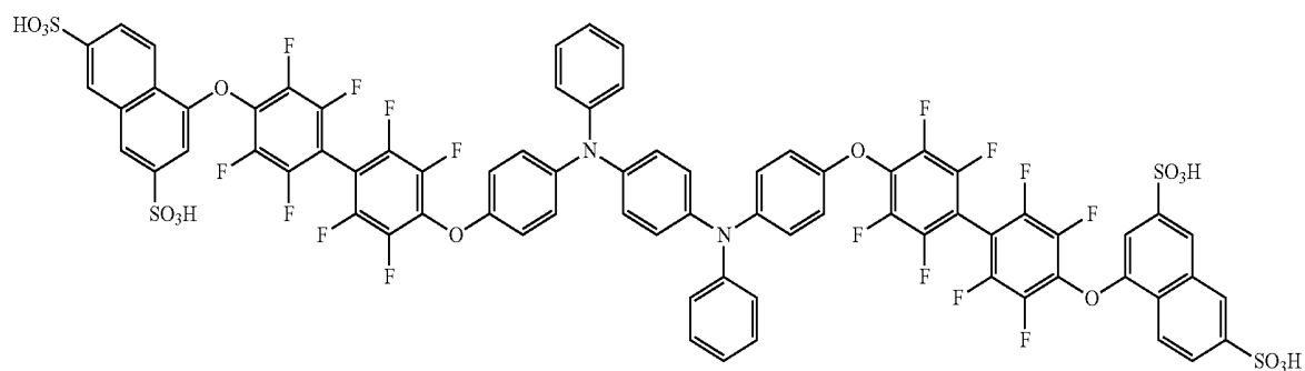
[Chemical Formula 1-4]
