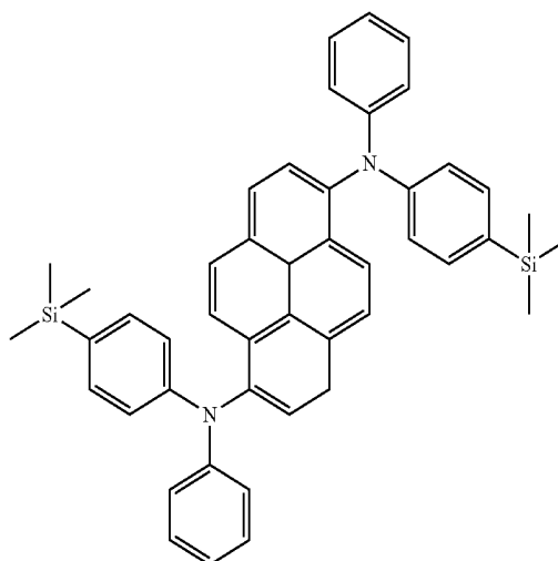
[Compound EM-2]
