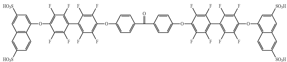
[Chemical Formula 1-2]
