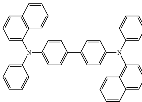
[Compound HT-1]
