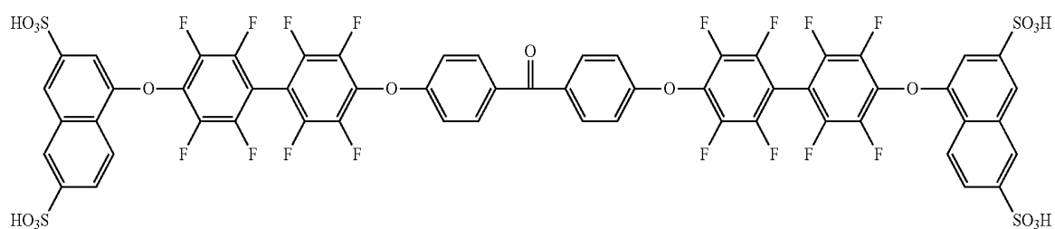
[Chemical Formula 1-3]
