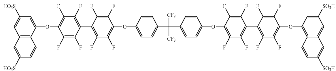
[Chemical Formula 1-1]
